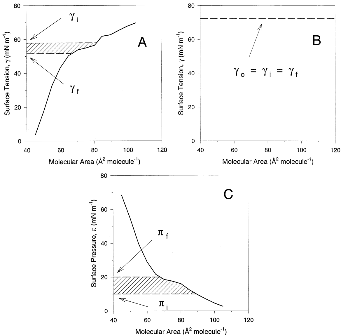
Fig. 5. A graphical illustration of the Goodrich-Gaines method of isotherm integration. (A) A plot of the integral defined by the equation: \int_{\gamma_f}^{\gamma_i} A(\gamma) d\gamma which illustrates the negative work done by the system as the barrier is compressed. The cross-hatched region represents the hypothetical region integrated between the surface tensions \gamma_i and \gamma_f by this integral. (B) A plot of the work done by the system to create the A/W interface outside of the barrier according to the integral: -\int_{\gamma_0}^{\gamma_0} A(\gamma) D\gamma . The value of this integral equates to zero since by the Goodrich-Gaines definition, \gamma_0 = \gamma_i = \gamma_f , where \gamma_0 is the surface tension of water (72 \text{mN/m} ). (C) The overall sum of the integrals presented in Fig. 5A, B, which illustrates the total work done by the system, defines the Goodrich-Gaines model of monolayer thermodynamics, and is represented by the following integral: \int_{\pi_i}^{\pi_f} A(\pi) d\pi . The cross-hatched area in the plot represents the hypothetical region integrated between the surface pressures \pi_i and \pi_f by this integral.
